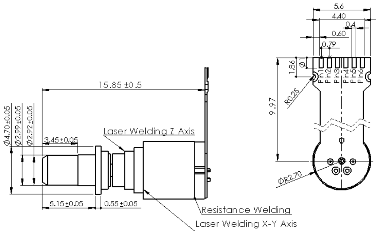
Flex Board PINOUT (Bottom View)
