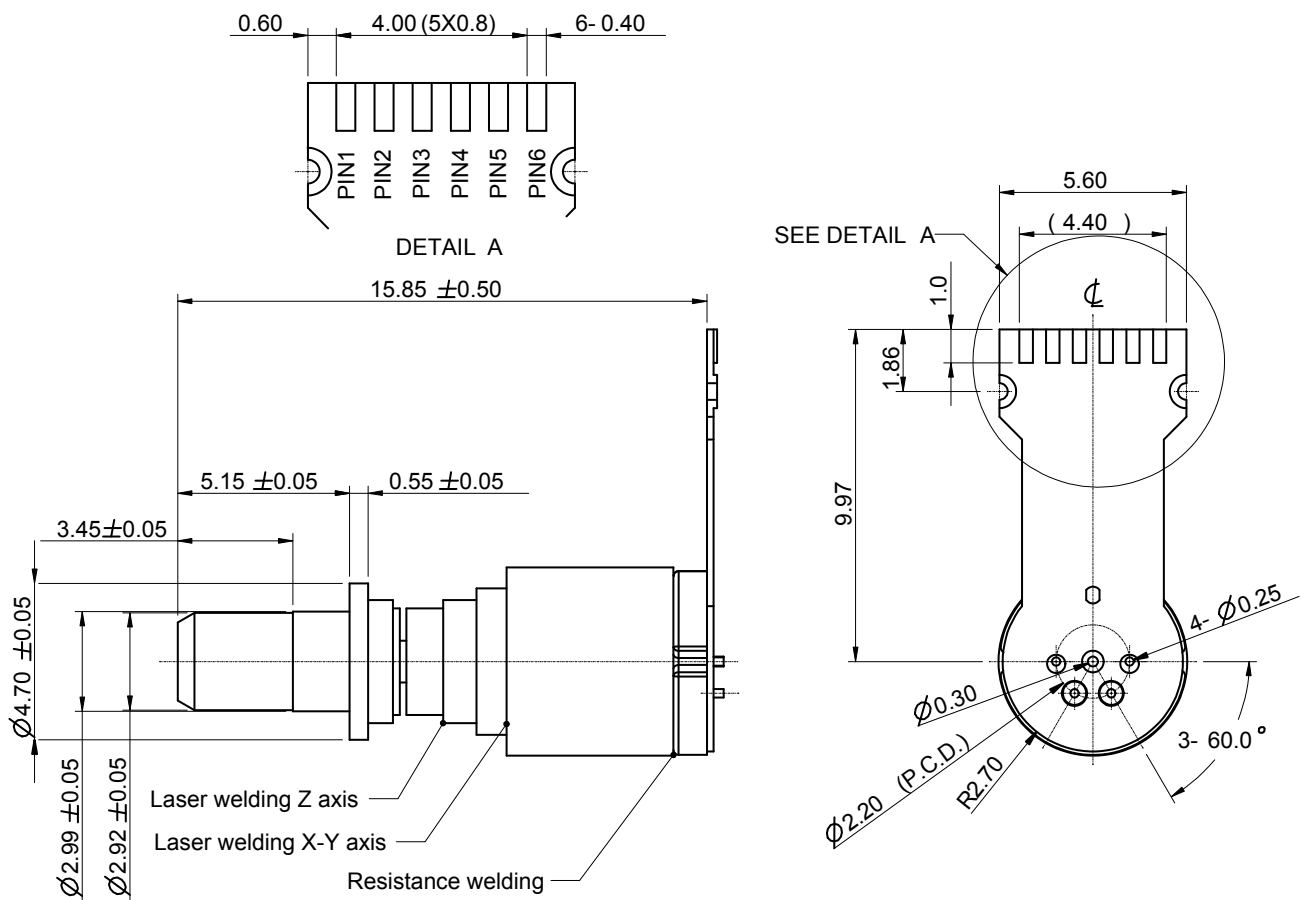
Flex Board PINOUT (Bottom View)
